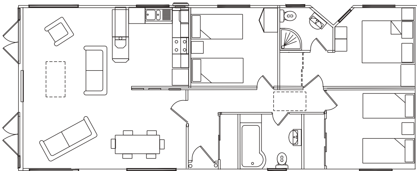
48' x 20' 2 Bedroom
